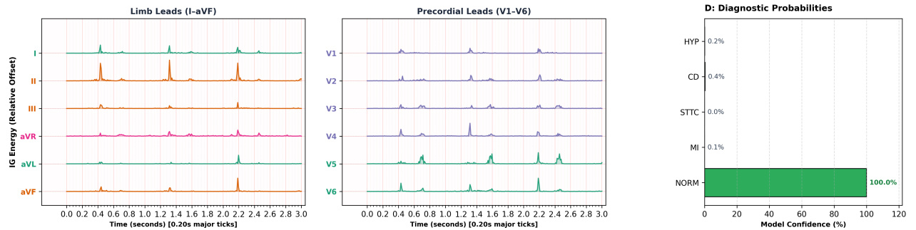
B: Axiomatic Integrated Gradients (Lead-Wise Instantaneous Attribution Energy | Synchronized 3.0s Zoom)
